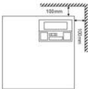
Enclosure Mounting
