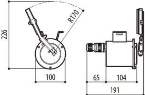
HCPWK Wiper Kit
