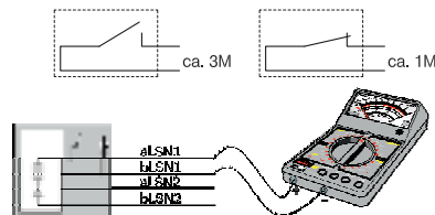
Fig.3 Checking the switching function of make contact (sabotage contact cannot be tested)
