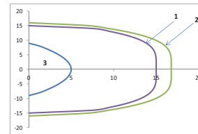
Fig.2 Distance diagram Magnet - magnet contact
