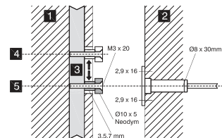
Fig.1 Front-end arrangement maximal axial misalignment ≤ 2mm
