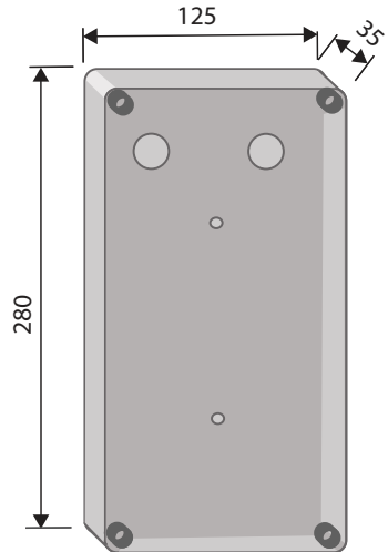
O.no. 1008098600 On wall master back box
