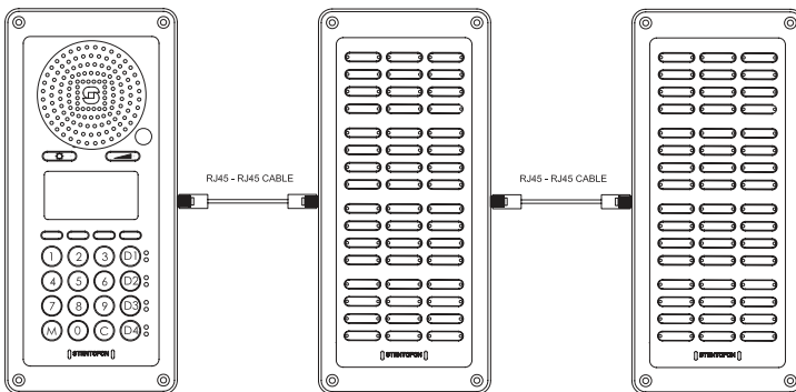
IP DAK 48 unit First module
